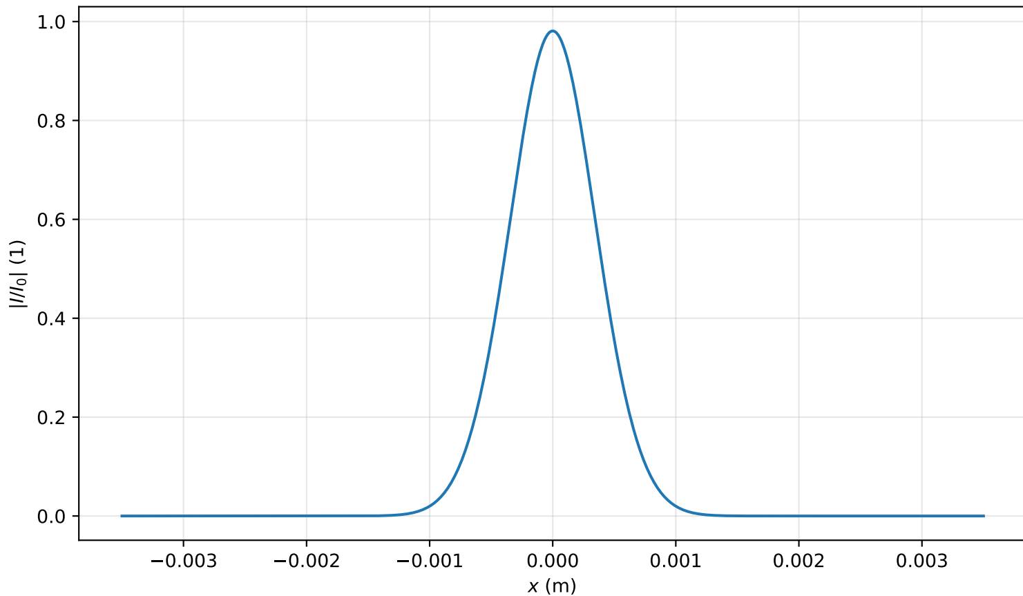
Intensity profile I(x, y = 0, z = 0.478m)/I_0 , P_{in}=0.2P_{cr} , artificial time
